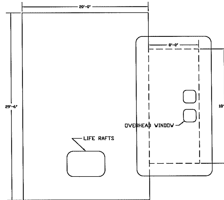
GENERAL ARRANGEMENT 04 LEVEL SCALE 1/4" = 1'-0"
