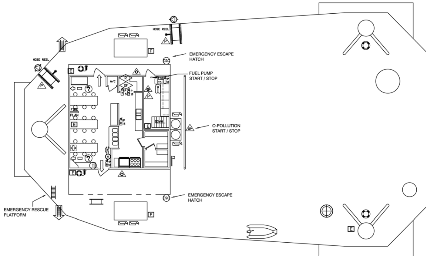
GENERAL ARRANGEMENT MAIN DECK
